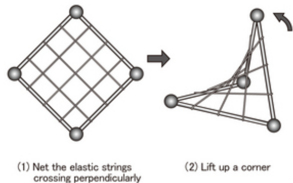
Fig. 2 Hyperbolic paraboloid
